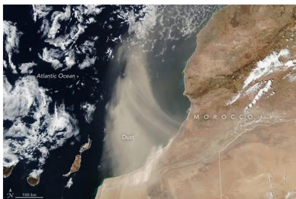
Figure 15 a) Satellite image showing a plume of Saharan dust streamed offshore from southern Morocco on August 24, 2024. Source: https://earthobservatory.nasa.gov/images/153246/dust-pours-off-the-moroccan-coast .
