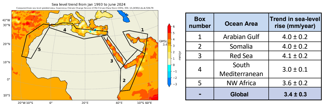
Figure 8. Spatial distribution of sea-level 10 trends in the five coastal regions of the Arab region covering the period from January 1993 to June 2024: Arabian Gulf (1), Somalia (2), Red Sea (3), South Mediterranean (4), and NW Africa (5). The global mean trend is 3.4 mm/year. The boxes represent subregions where the rates of area-averaged sea-level change are provided in Table 2.
